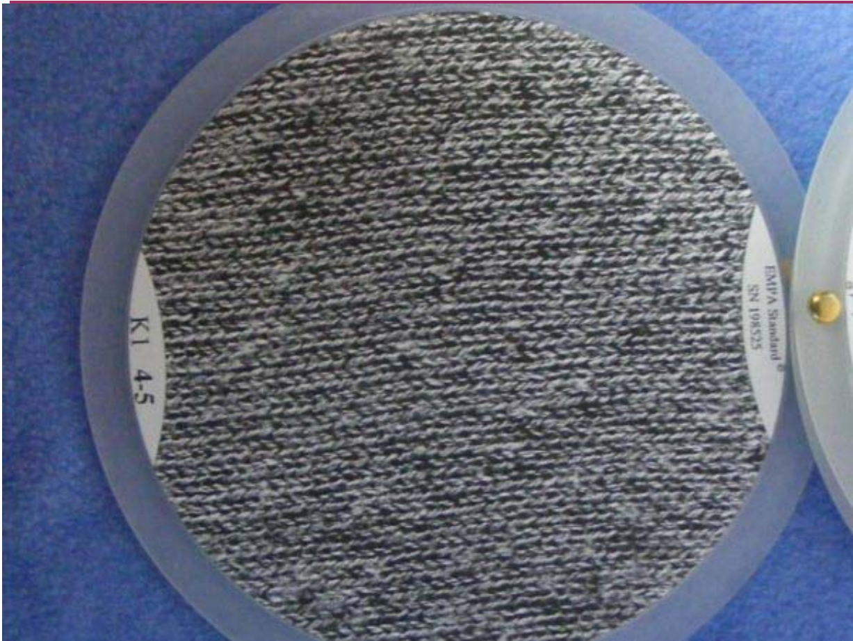
DETAILED PICTURE OF PHOTOGRAPHIC STANDARDS FOR KNITTED FABRIC
